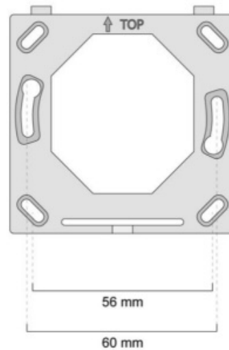
Fig.3. mounting plate
