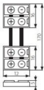
CONNECTOR 8-CPC
