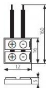
CONNECTOR 8-CP
