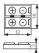
CONNECTOR 8
